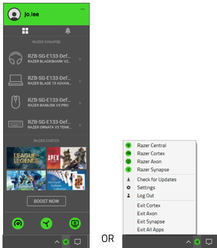
Left-click action
